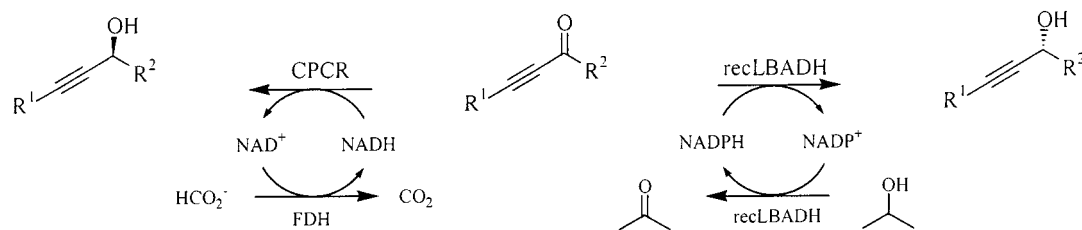
Scheme 2. Enzymatic reductions with cofactor-regeneration
