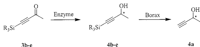
Scheme 3. Synthesis of enantiopure 3-butyn-2-ol ( 4a )
